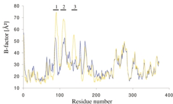
Fig. 7. B -factors of the C \alpha atoms of the A- (yellow) and B- (blue) monomer of T.l.MalK. Regions of high asymmetry are marked by bars and labelled with numbers. The A-chain is significantly more disordered in the 'lid' region (1), the loop between helices 2 and 3 (2) and the signature motif region (3). The regulatory domains have fairly similar B -factors.
