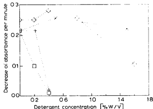
Fig. 2. Decrease per minute in the absorbance at 340 nm after addition of 8 \mu\text{g} of SR vesicles to 3 ml of the assay medium plotted as a function of the detergent concentration in the assay medium. ○, ES-8-H; □, ES-10-H; +, ES-11-H; ×, ES-12-H. The cmc values are given in Table I.
