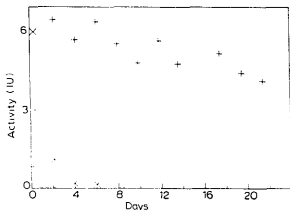
Fig. 6. ATPase activity of the hydroxyapatite preparation as a function of time (for equilibration, buffer B2 was used with 10 mM phosphate and 500 \mu\text{g} M EGTA added and for elution a phosphate gradient was used as given in Results). Values are shown upon storage at 4°C (+) and upon storage at room temperature (x).
