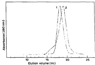
Fig. 4. Gel filtration of solubilized SR vesicles. In the presence of 50 \mu\text{M} \text{Ca}^{2+} the protein band elutes at 18.2 ml, without \text{Ca}^{2+} in the presence of 500 \mu\text{M} EGTA the protein band elutes at 19.0 ml.
